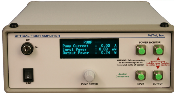
LNTFA-xx model with power monitor option
