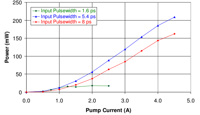
SHG Output Power: Input Pulswidth Dependence Input: FFL, 20 MHz, 1550 nm
