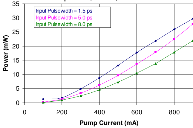
SHG Output Power: Input Pulswidth Dependence Input: FFL, 20 MHz, 1550 nm
