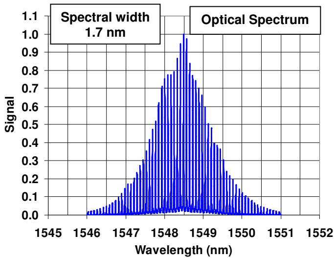
Optical spectrum and Autocorrelation at 10 GHz, pulsewidth 1.6 ps
